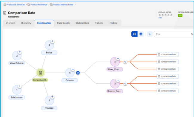
Lineage from conceptual data to business process, policy and through to physical data (tables and attributes).
